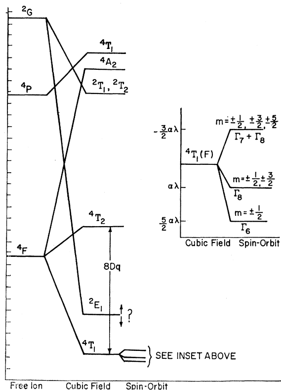
FIG. 1. A partial energy-level diagram for 3d^7 ions in MgO due to the combined action of the octahedral crystal field of a point-charge lattice and spin-orbit coupling. For \text{Fe}^{1+} , the location of the {}^2E_1 level is uncertain but it is likely to be shifted below the {}^4T_2 state, as discussed in the text. The {}^4T_1 ground-state spin-orbit levels, shown on the right, are labeled with their symmetry properties and eigenvalues. The value of \alpha is approximately \frac{2}{3} , and the spin-orbit coupling constant \lambda is negative.
